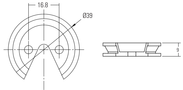
Mounting plate
