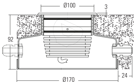
/485N Concrete housing with 1x PG9 IP67 gland
